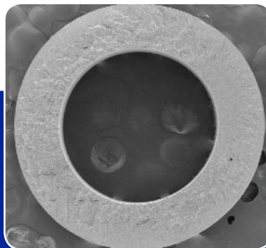
Figure 5: Cross section of PVDF membrane x40
